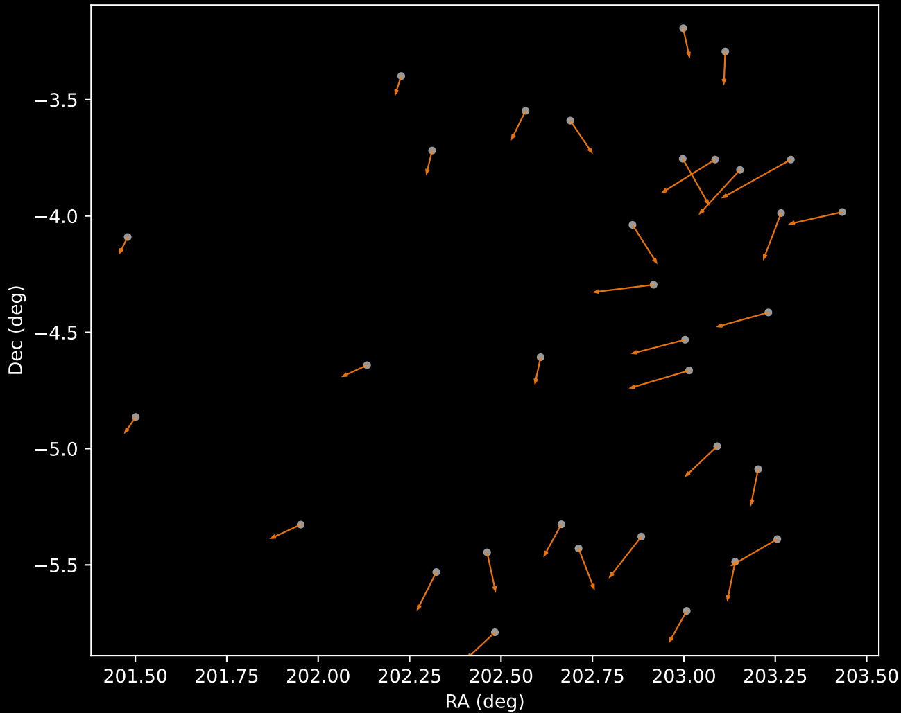
APOGEE DR17 Cluster 2 Proper Motion Vectors (n=33)
