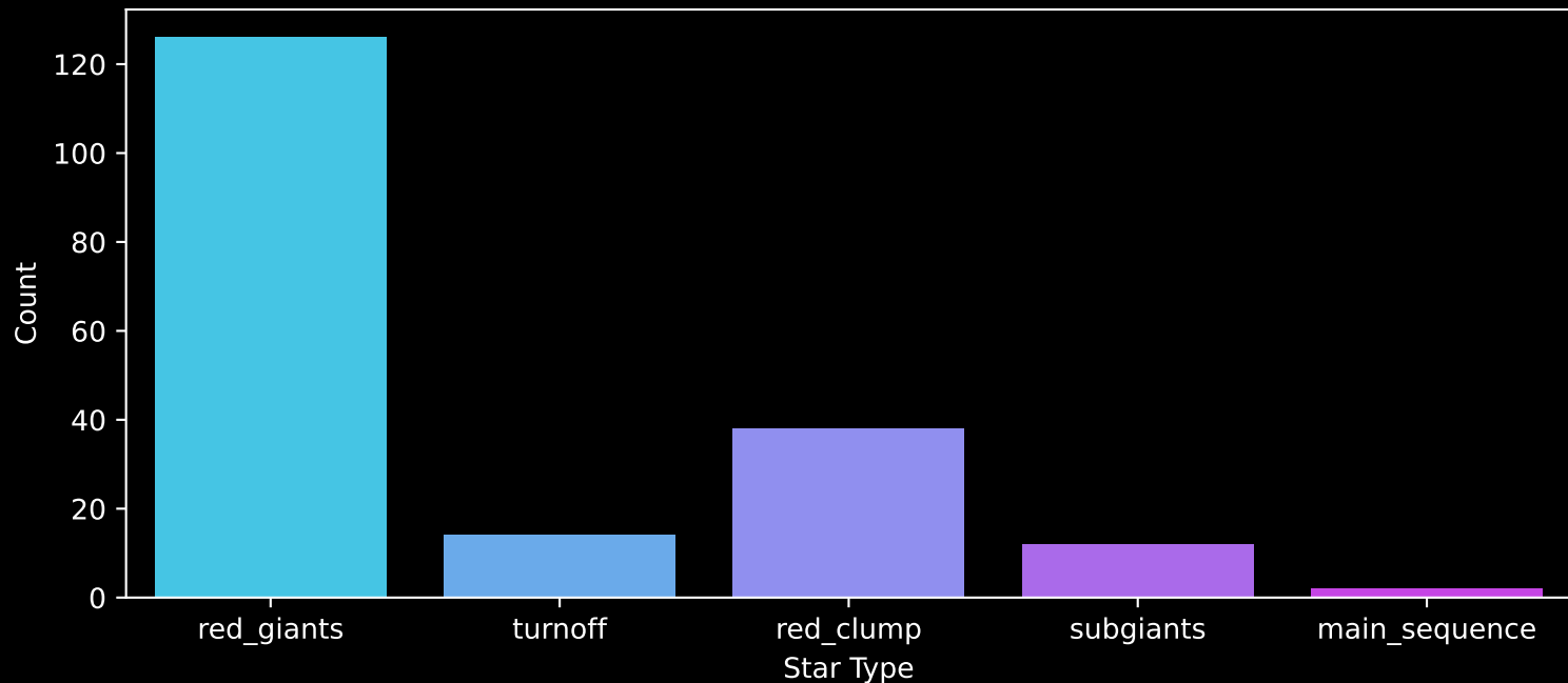
APOGEE DR17 Field: [COROTA2] Count plot of Star Type
