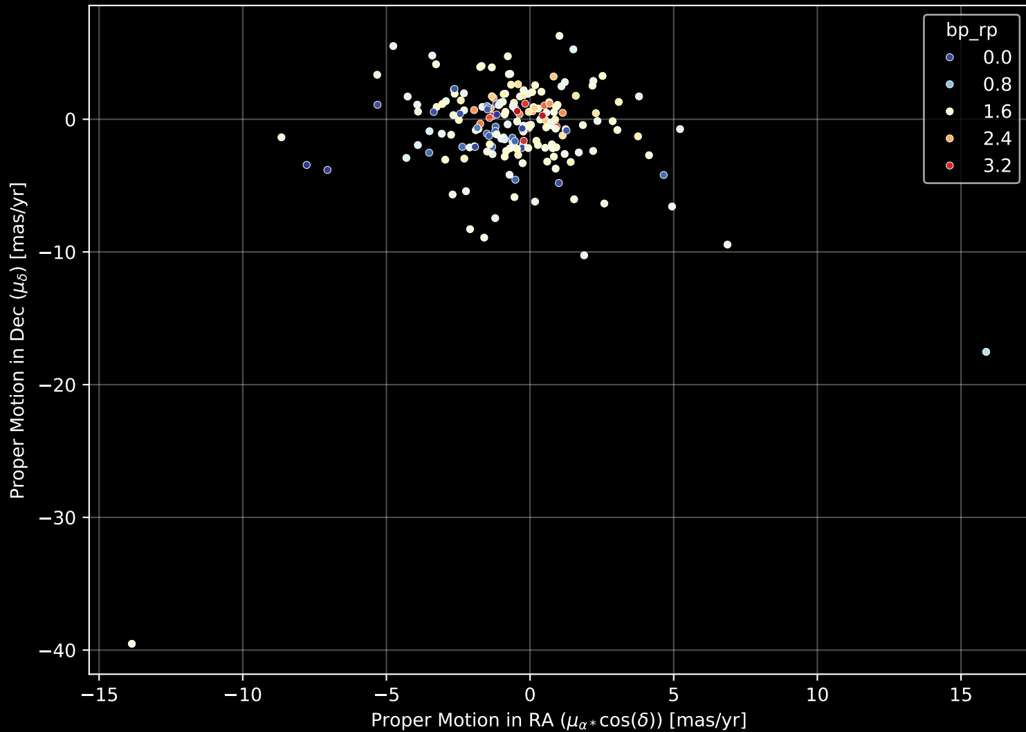
APOGEE DR17 Field: [COROT A2] Proper Motion Diagram (n= 192)
