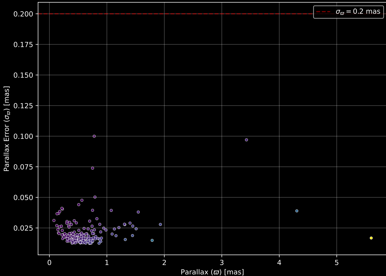
APOGEE DR17 Field: [COROTA2] Parallax Quality (n= 192)
