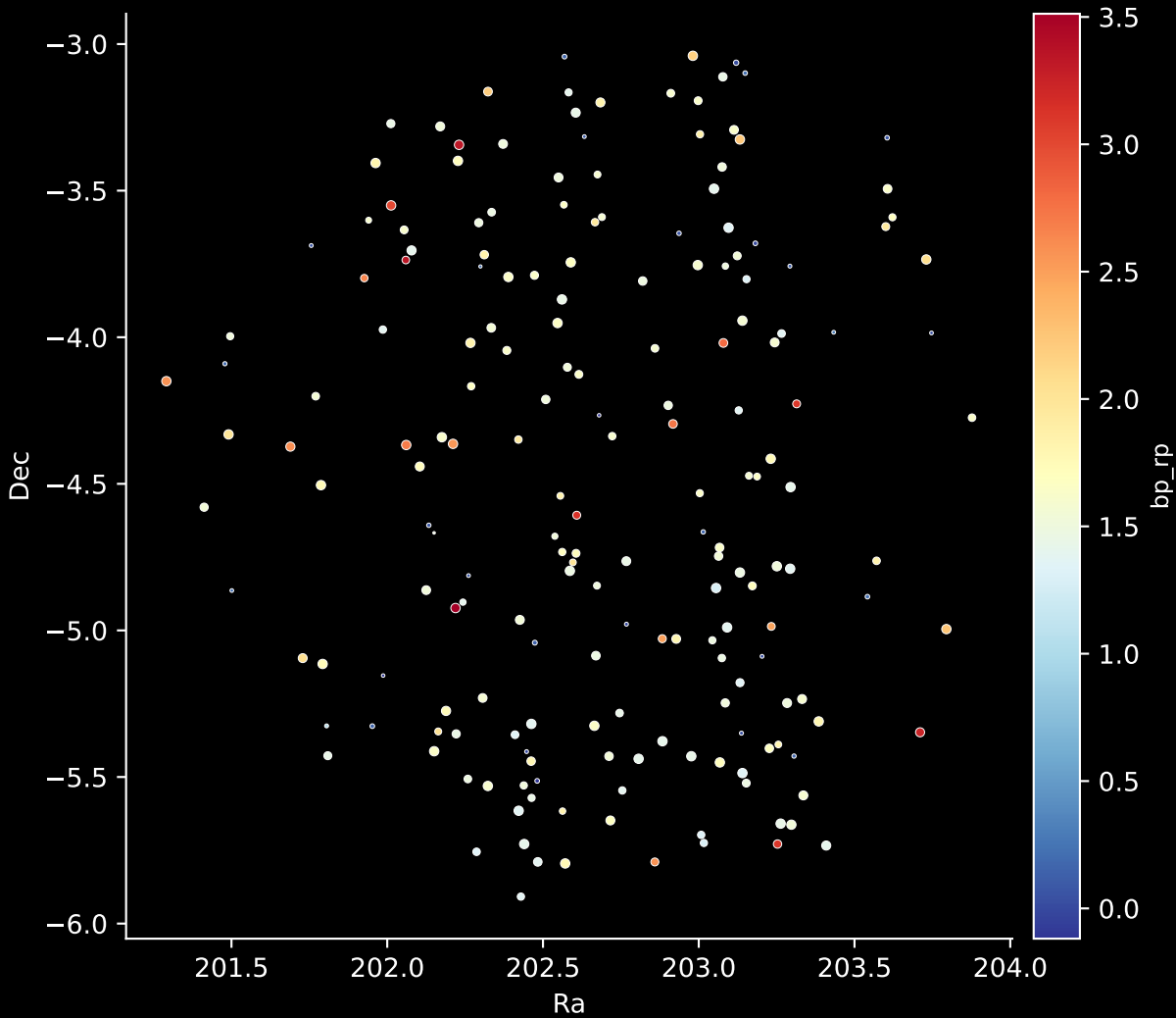
APOGEE DR17 Field: [COROTA2] Stars: 192
