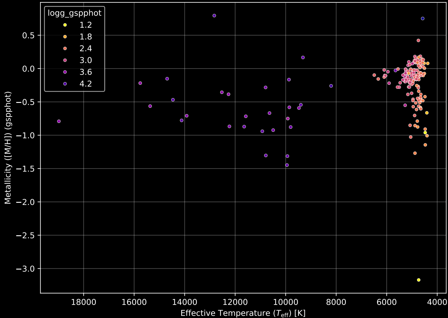
APOGEE DR17 Field: [COROTA2] Stellar Population Parameters (n= 192)
