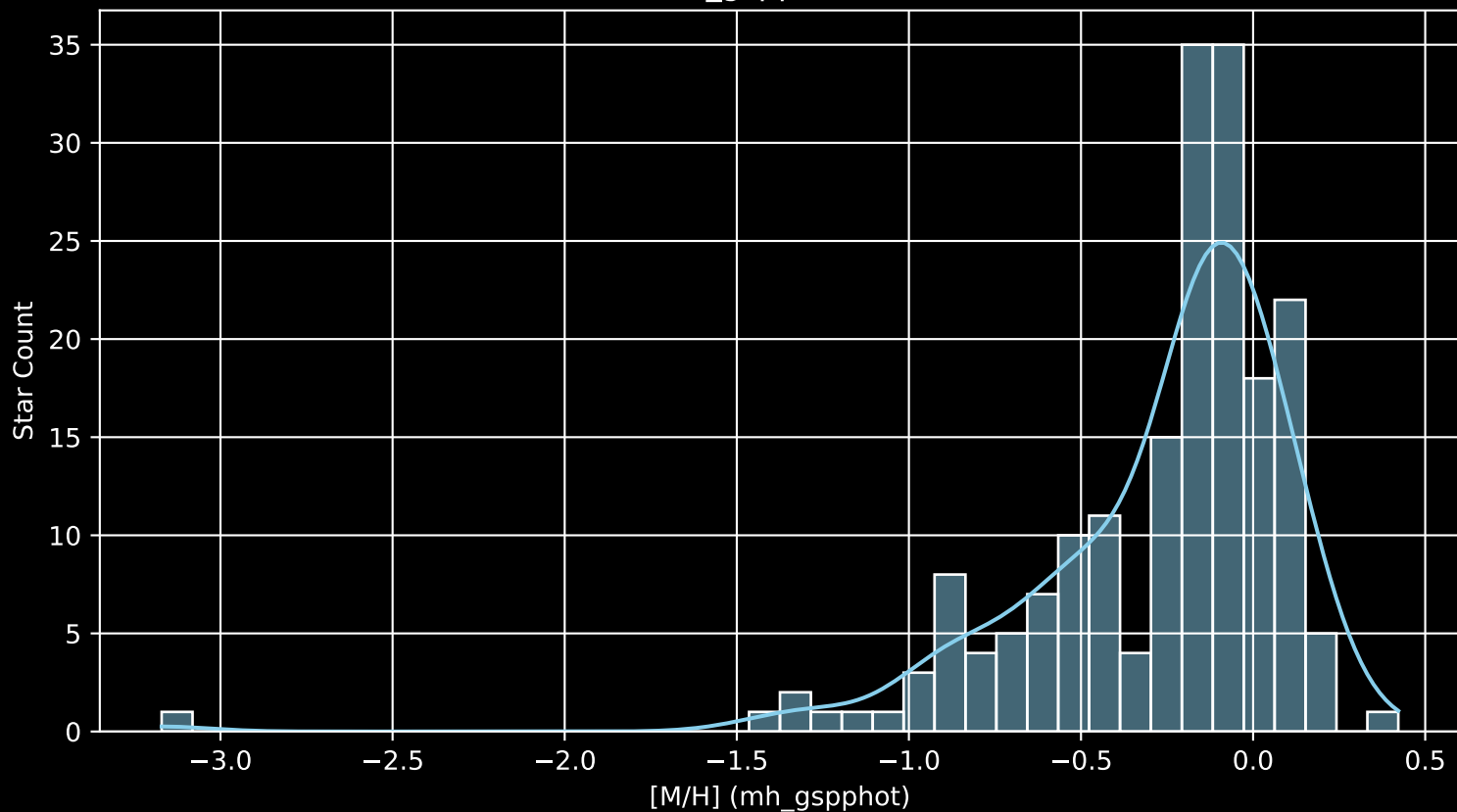
APOGEE DR17 Field: [COROTA2 [M/H] (mh_gspphot) (n= 190)
