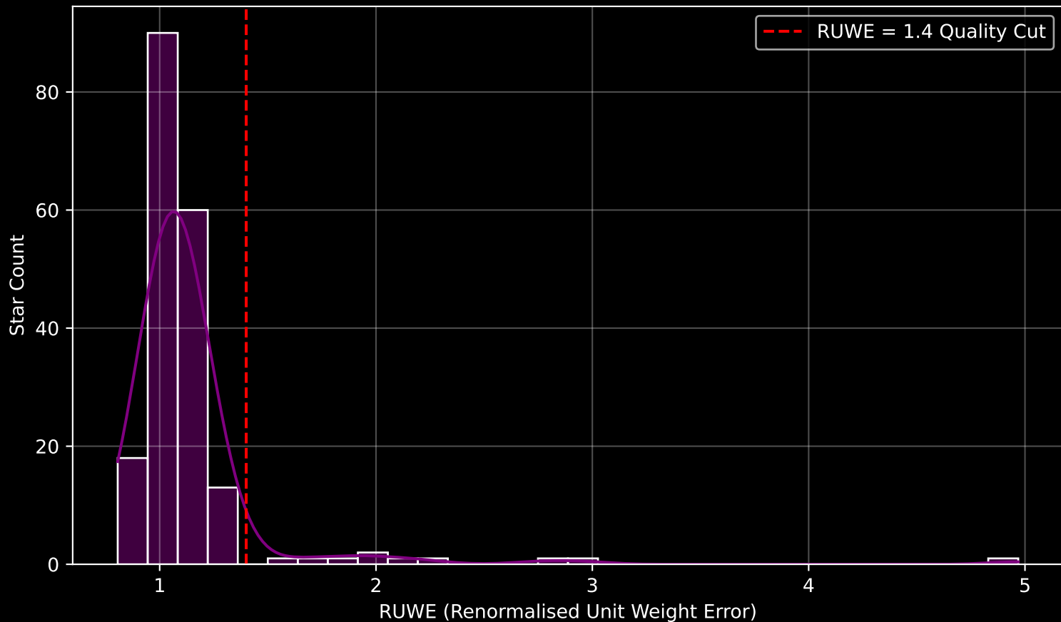
GAPOGEE DR17 Field [COROTA2] RUWE Distribution (n= 191)
